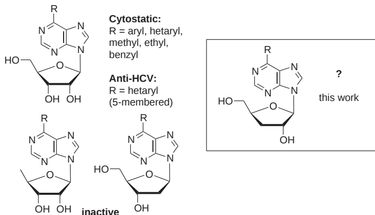
CHART 1 6-Substituted purine nucleosides
